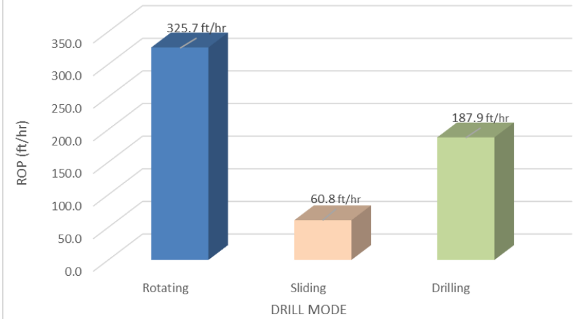
12 1/4" INTERMEDIATE HOLE NET ROP
